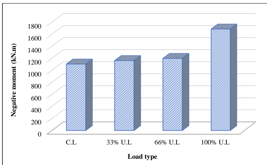
Figure 19. Influence of load type variation on negative moments
