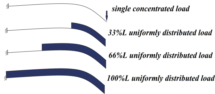
Figure 18. Distribution of the uniform load on the beams by the method of thirds
