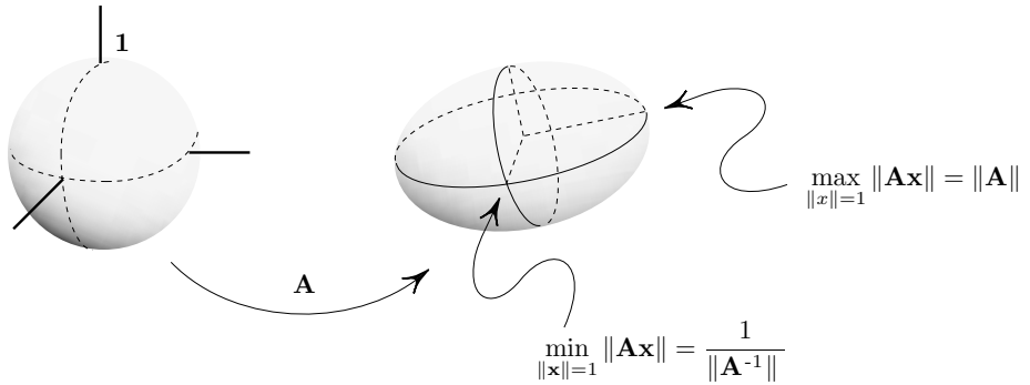
FIGURE 5.2.1.1. THE INDUCED MATRIX 2-NORM IN \mathbb{R}^3 .
