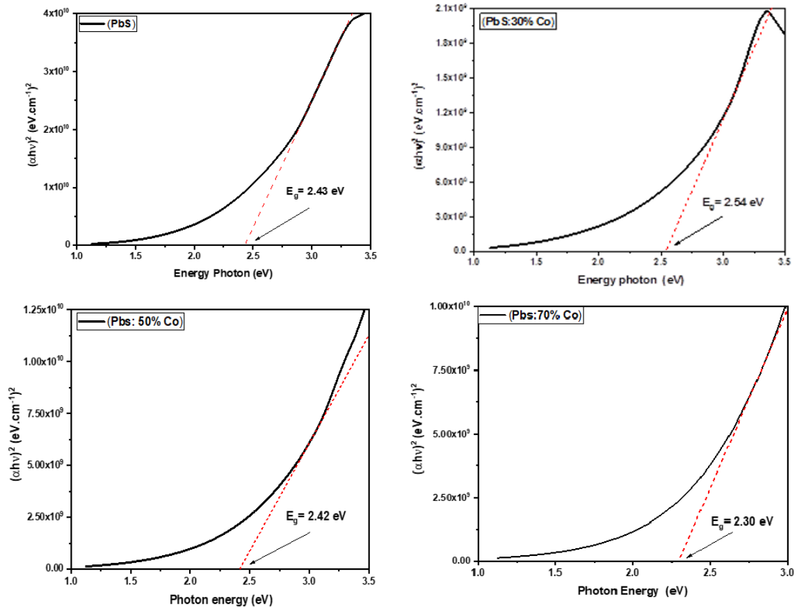
Figure 7: The relation between (\alpha h\nu)^2 and (h\nu) of pure and mixed thin films at different ratios of Co
