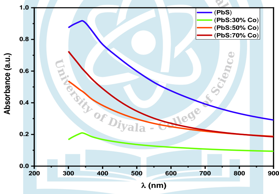
Figure 5: Absorbance versus wavelength of pure and mixed thin films with different ratios of Co.
