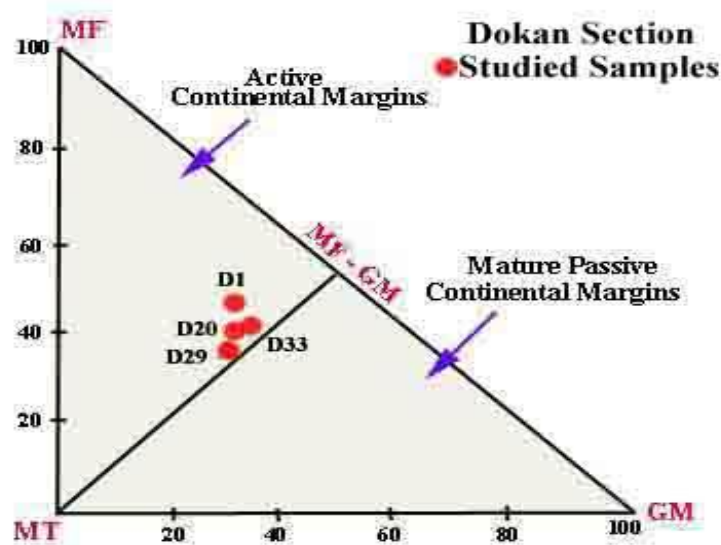
Figure 6: Interrelationship of the Dokan sandstone's MF-MT-GM suites, following [14].
