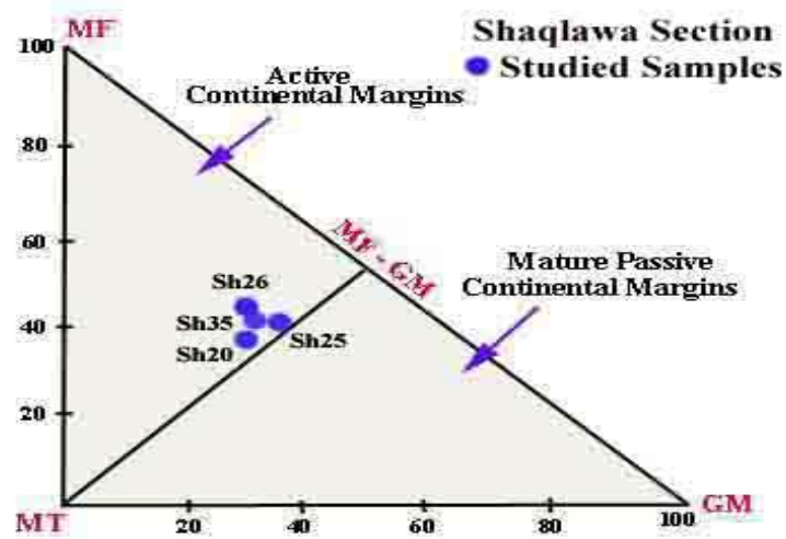
Figure 5: Interrelationship of the Shaqlawa sandstone's MF-MT-GM suites, following [14].
