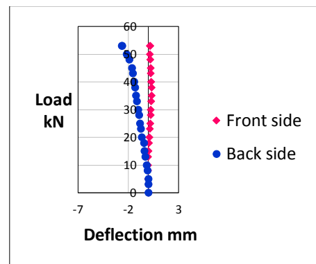
Figure 17: Cross-section behavior of the specimen BT7
