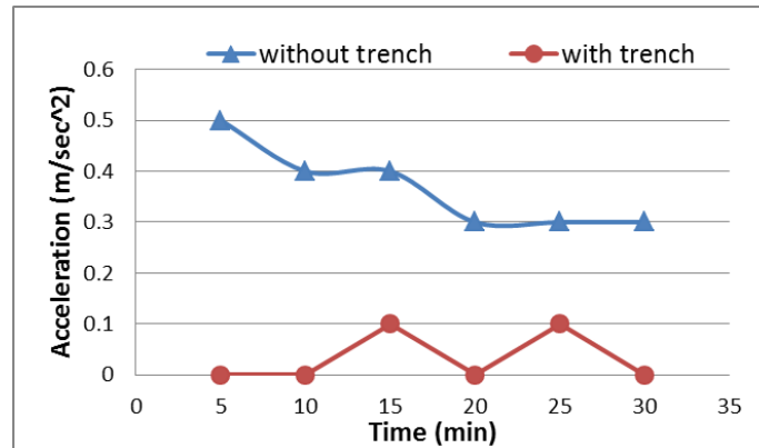
Fig 14. Variation of acceleration with time at frequency (8 Hz) for (length=3B, depth=B, thickness=0.5 B) at dry state to low density polyethylene
