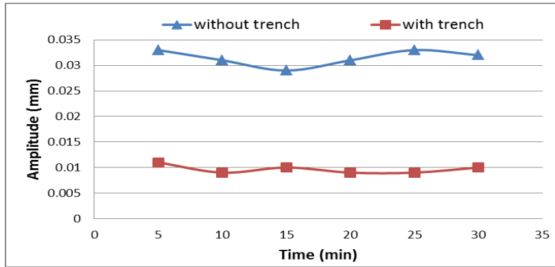
Fig 6. Variation of amplitude with time at frequency(8Hz) for (length=3B, depth=B, thickness=0.5 B) at dry state styropor
