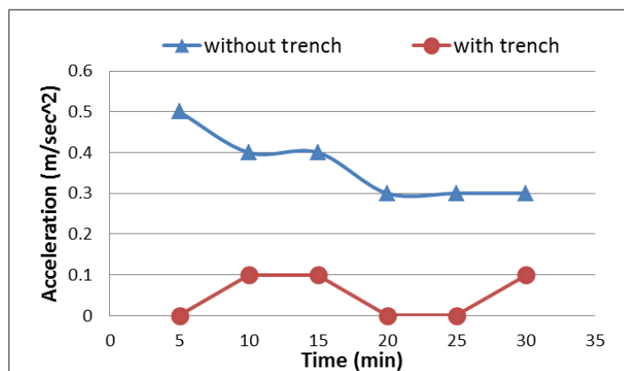
Fig 12. Variation of acceleration with time at frequency (8 Hz) for (length=3B, depth=B, thickness=0.5 B) at dry state to styropor
