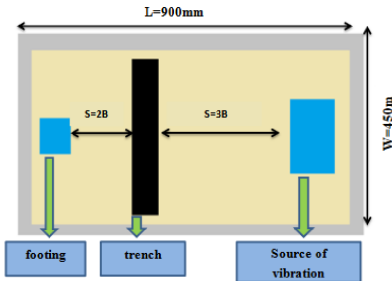
Fig 1. Layout of experimental model
