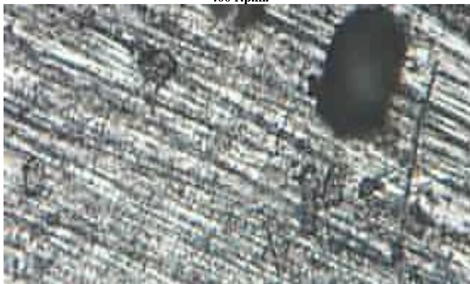
Fig. 23 Corrosion on surface of carbon steel in kerosene + 10% V NaCl with CO 2 at 328 K and 400 r.p.m.
