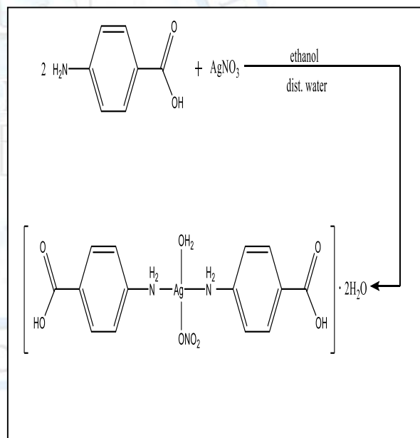
Scheme -4: Synthesis route of complex-4: [Ag(PAB)_2(NO_3)(H_2O)] \cdot 2H_2O .
