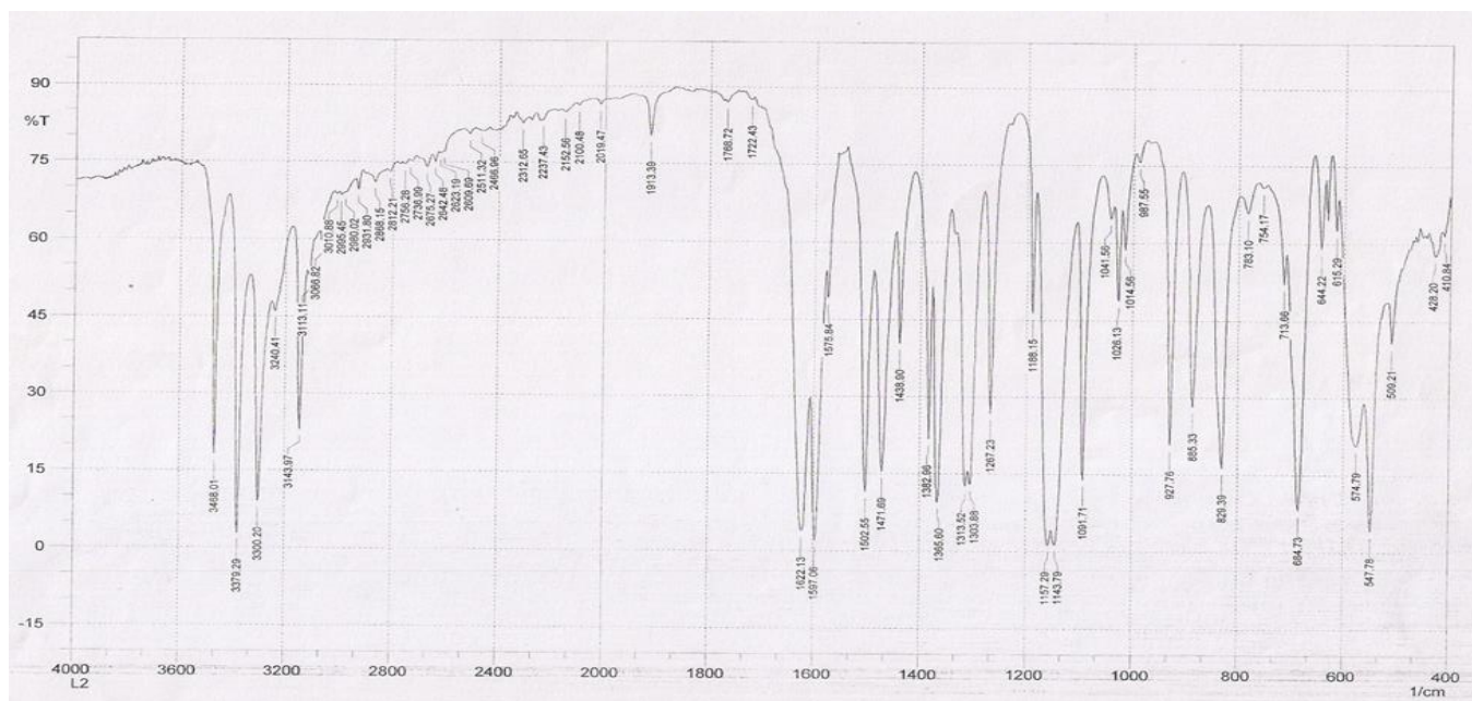
Fig.2 : FT-IR spectrum of complex-1: [Ag(SMZ)(NO 3 )(H 2 O)]. H 2 O.
