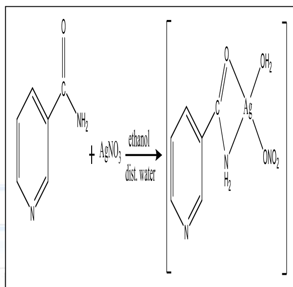
Scheme -2: Synthesis route of complex-2: [Ag(NAM)(NO_3)(H_2O)] .
