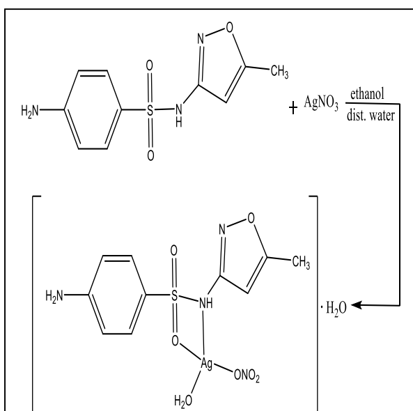
Scheme -1: Synthesis route of complex-1: [Ag(SMZ)(NO_3)(H_2O)] \cdot H_2O .
