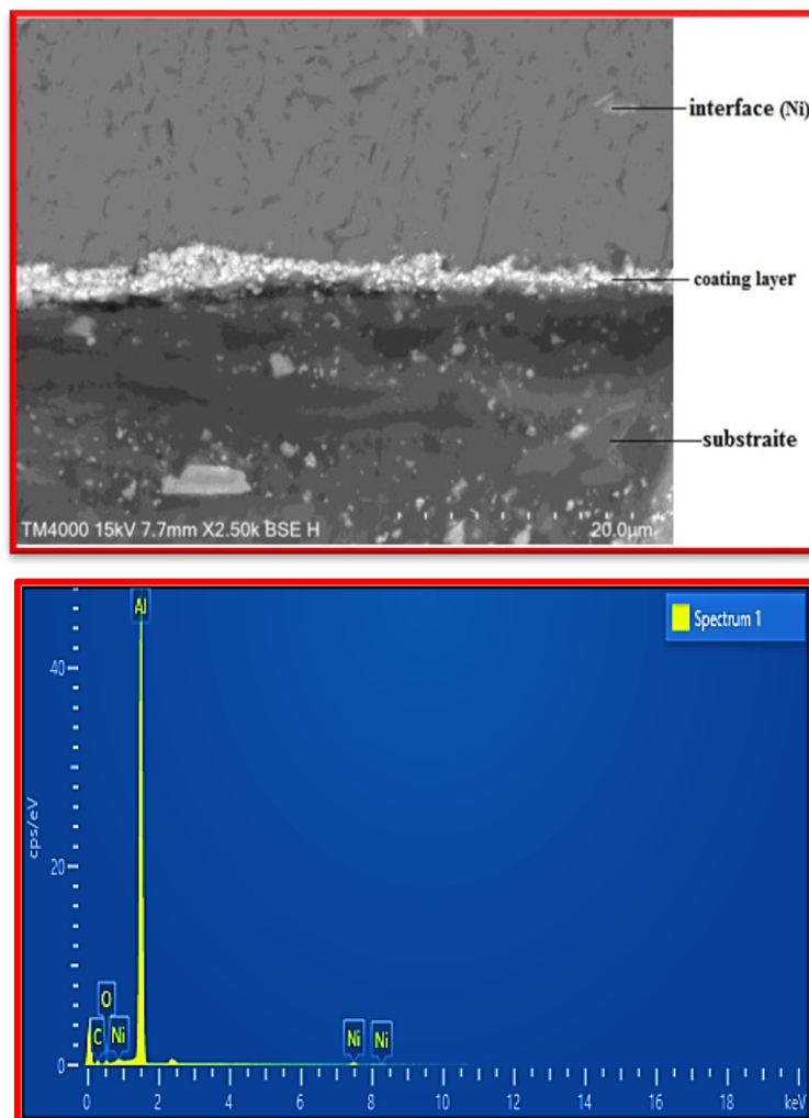
Figure 1. Ni - \text{Al}_2\text{O}_3 nanocomposite coating with alumina 4 g/L concentration, EDS & cross-sectional SEM image
