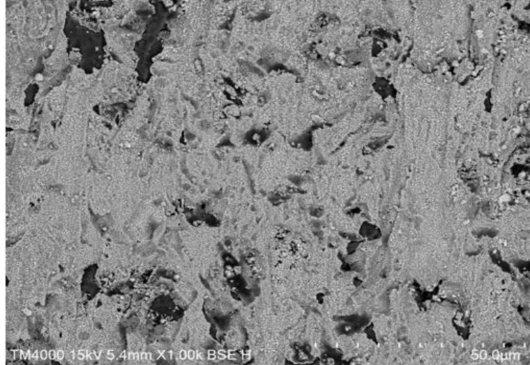
Figure 2: SEM images of nanocomposite coating Ni-Al 2 O 3 at Al 2 O 3 4 g/L nanoparticle concentration
