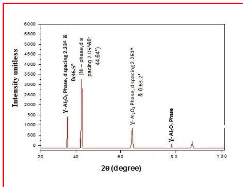
Figure 3. XRD chart of Ni- Al 2 O 3 nanocomposite coating
