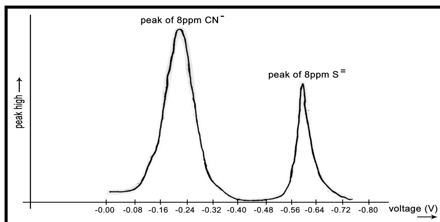
Figure 3 polarogram of cyanide and sulfide ions in support (boric acid + KOH) using Dp mode using differential puls polarography.
