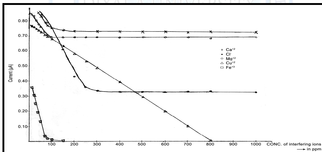
Figure 5 Effect of the interfering ions on sulfide ion determination using the polarographic method.
